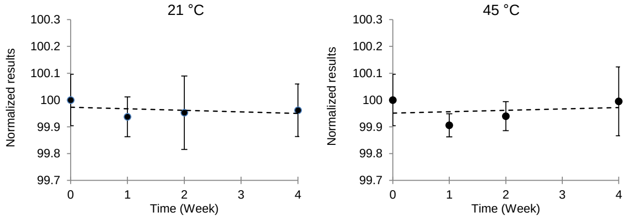
Figure A2.4. STS Plots for UME CRM 2213 (Co) at +21 °C and +45 °C
