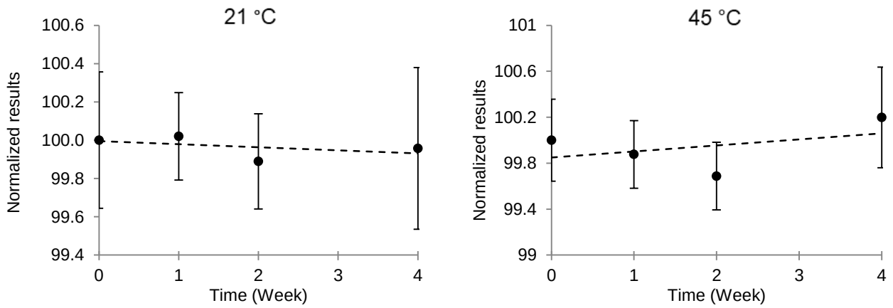
Figure A2.2. STS Plots for UME CRM 2210 (Ca) at +21 °C and +45 °C
