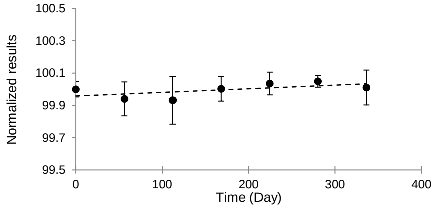
Figure A3.4. LTS Plot for UME CRM 2213 (Co) at +21 °C
