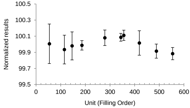
Figure A1.7. Homogeneity Plot for UME CRM 2236 (Na)
