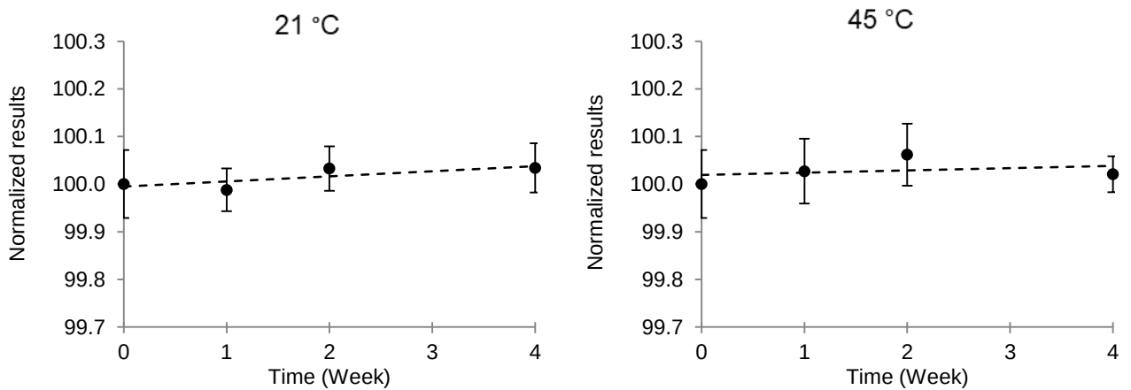
Figure A2.6. STS Plots for UME CRM 2229 (K) at +21 °C and +45 °C
