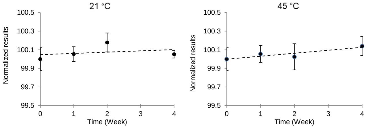
Figure A2.5. STS Plots for UME CRM 2216 (Cu) at +21 °C and +45 °C
