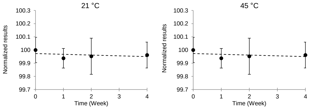
Figure A2.3. STS Plots for UME CRM 2211 (Cd) at +21 °C and +45 °C
