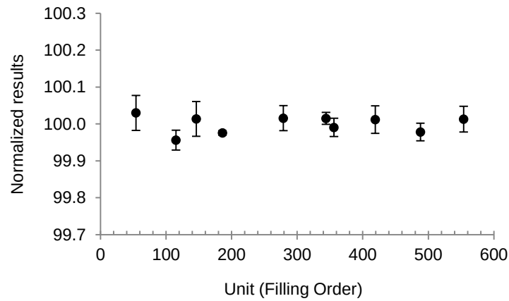
Figure A1.6. Homogeneity Plot for UME CRM 2229 (K)
