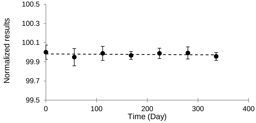
Figure A3.1. LTS Plot for UME CRM 2203 (As) at +21 °C
