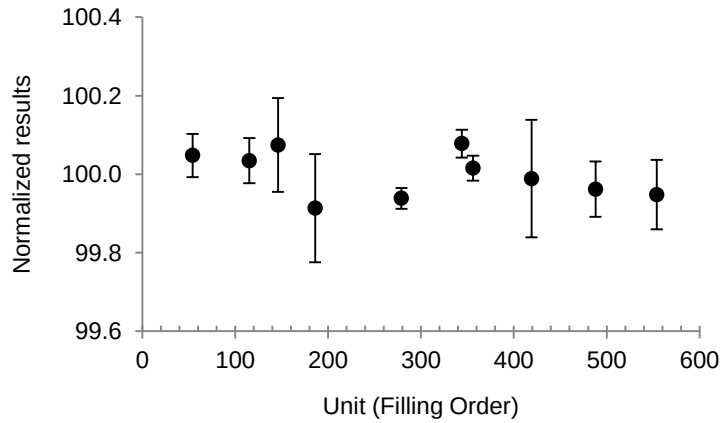
Figure A1.3. Homogeneity Plot for UME CRM 2211 (Cd)
