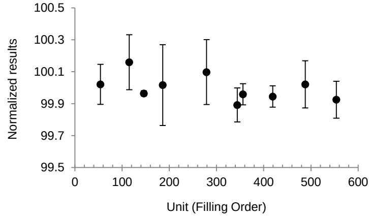
Figure A1.4. Homogeneity Plot for UME CRM 2213 (Co)
