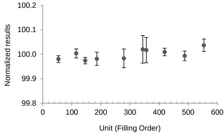
Figure A1.1. Homogeneity Plot for UME CRM 2203 (As)
