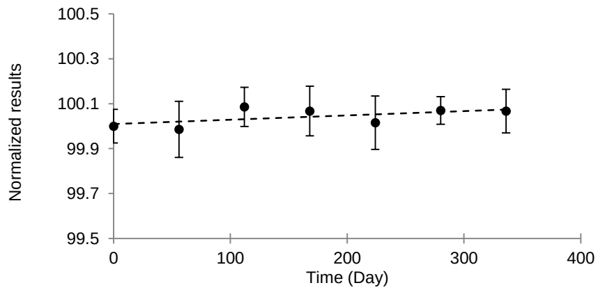
Figure A3.6. LTS Plot for UME CRM 2229 (K) at +21 °C
