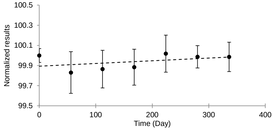
Figure A3.7. LTS Plot for UME CRM 2236 (Na) at +21 °C
