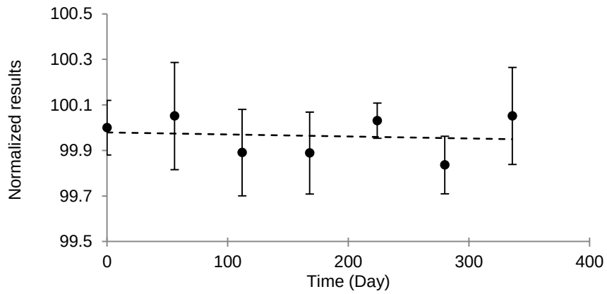
Figure A3.2. LTS Plot for UME CRM 2210 (Ca) at +21 °C
