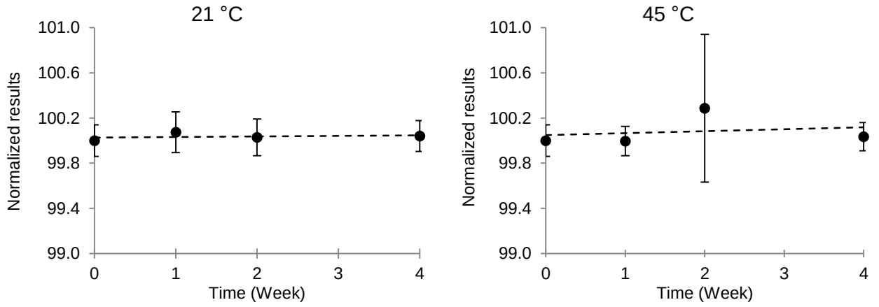
Figure A2.8. STS Plots for UME CRM 2270 (Zn) at +21 °C and +45 °C
