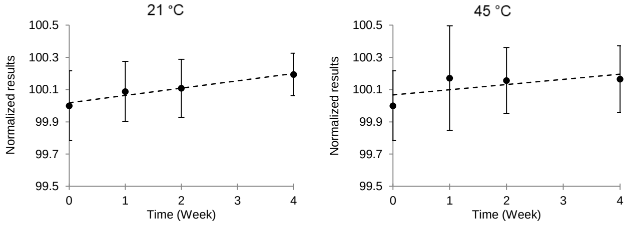
Figure A2.7. STS Plots for UME CRM 2236 (Na) at +21 °C and +45 °C
