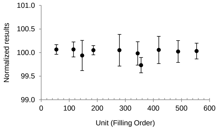
Figure A1.2. Homogeneity Plot for UME CRM 2210 (Ca)
