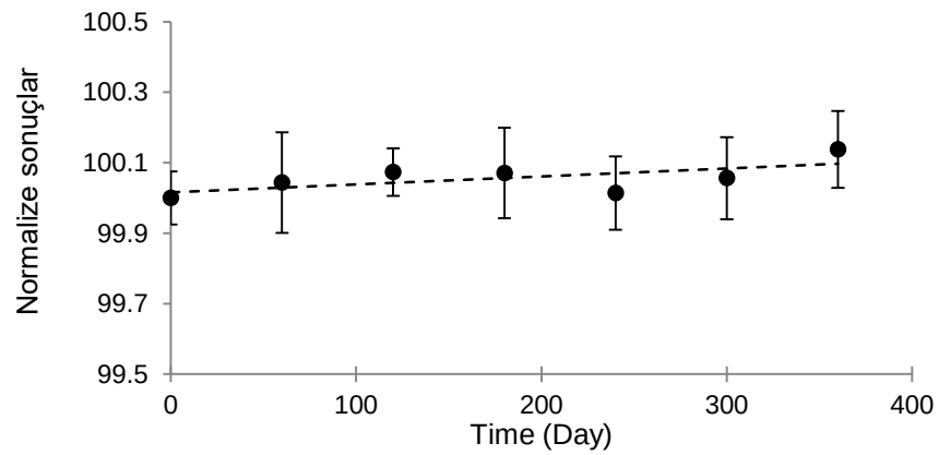
Figure A3.3. LTS Plot for UME CRM 2211 (Cd) at +21 °C
