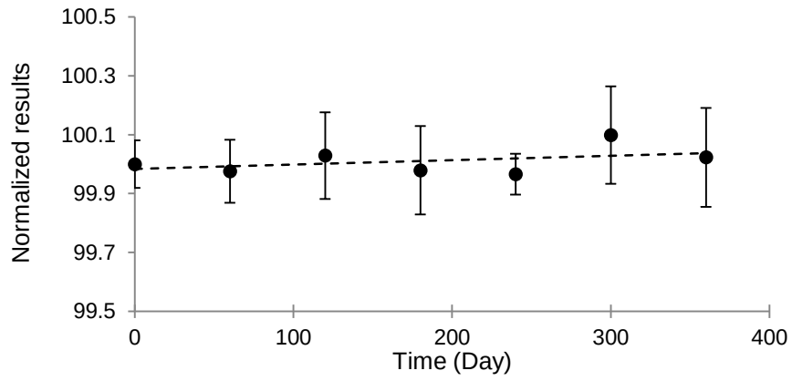
Figure A3.8. LTS Plot for UME CRM 2270 (Zn) at +21 °C
