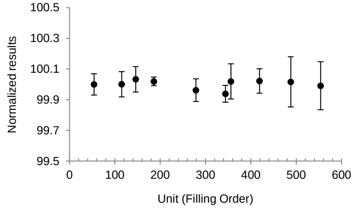
Figure A1.5. Homogeneity Plot for UME CRM 2216 (Cu)
