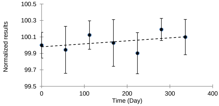
Figure A3.5. LTS Plot for UME CRM 2216 (Cu) at +21 °C
