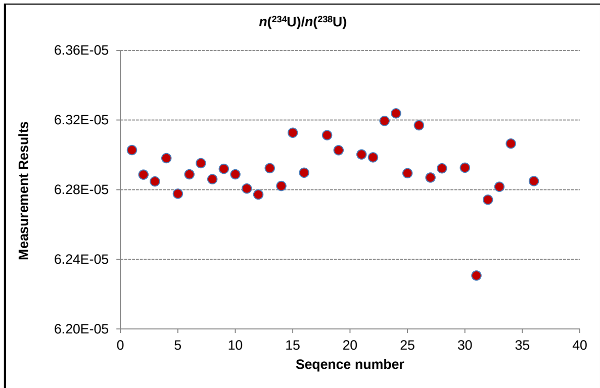
Figure A3.8. Long-term stability at +21 °C for °C for n(^{234}\text{U})/n(^{238}\text{U})
