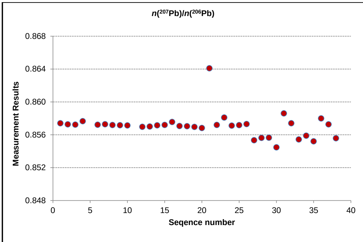
Figure A3.6. Long-term stability at +21 °C for n(^{207}\text{Pb})/n(^{206}\text{Pb})
