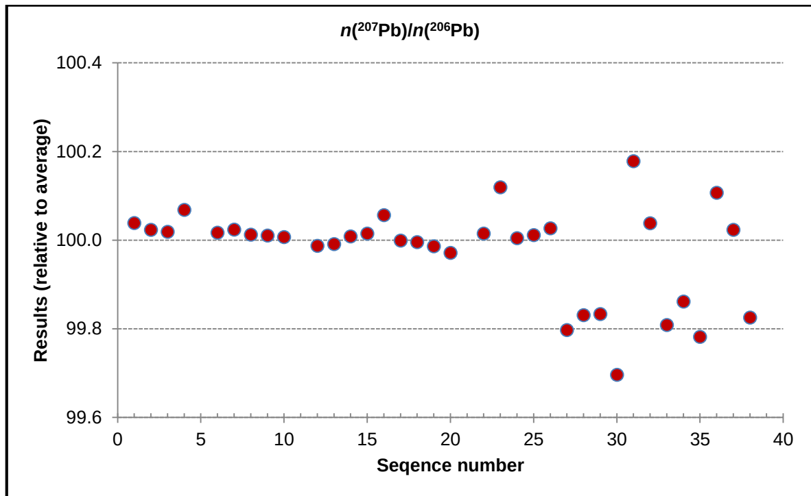
Figure A1.6. Homogeneity graphs for n(^{207}\text{Pb})/n(^{206}\text{Pb})
