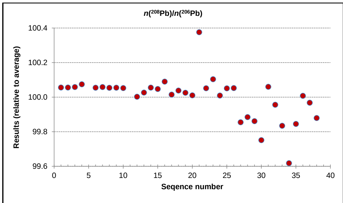
Figure A1.7. Homogeneity graphs for n(^{208}\text{Pb})/n(^{206}\text{Pb})
