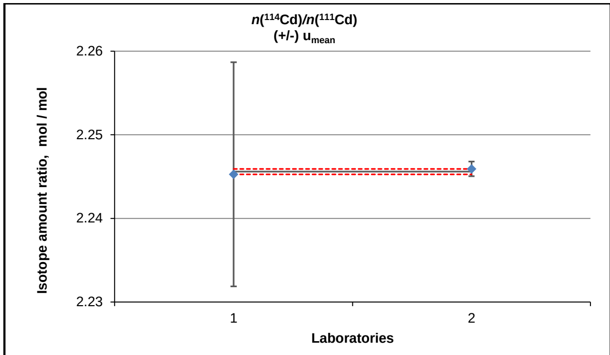
Figure A4.3. Interlaboratory study results for characterization of n(^{114}\text{Cd})/n(^{111}\text{Cd})
