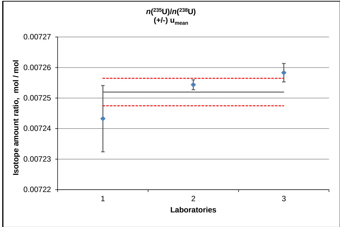
Figure A4.9. Interlaboratory study results for characterization of n(^{235}\text{U})/n(^{238}\text{U})
