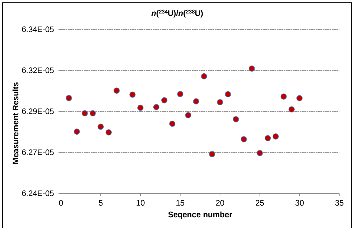
Figure A2.8. Short-term stability at +45 °C for n(^{234}\text{U})/n(^{238}\text{U})
