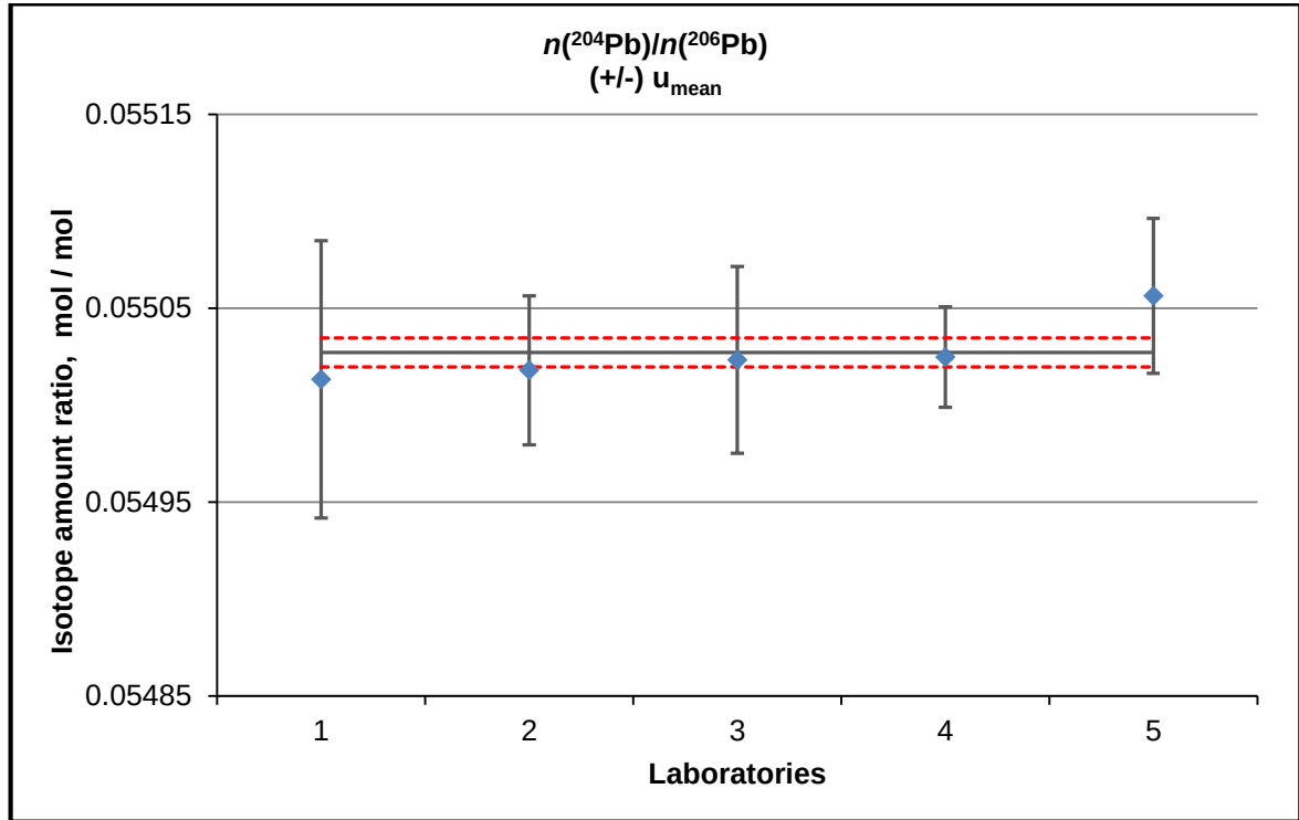
Figure A4.5. Interlaboratory study results for characterization of n(^{204}\text{Pb})/n(^{206}\text{Pb})
