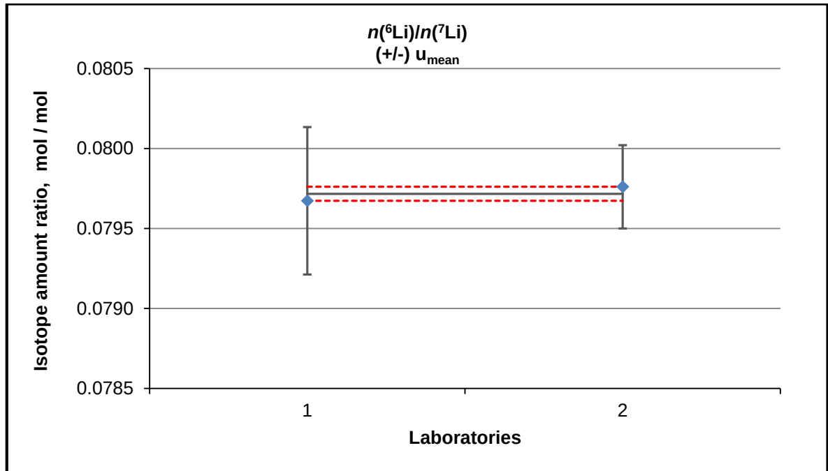
Figure A4.4. Interlaboratory study results for characterization of n(^6\text{Li})/n(^7\text{Li})
