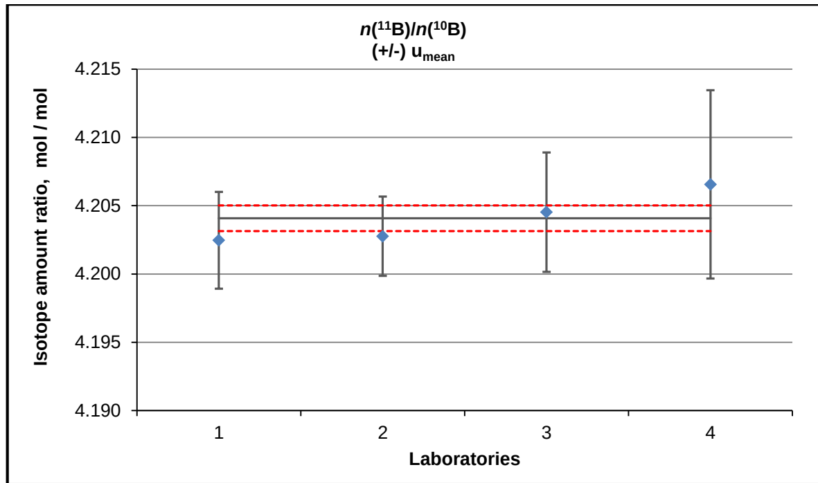
Figure A4.1. Interlaboratory study results for characterization of n(^{11}\text{B})/n(^{10}\text{B})
