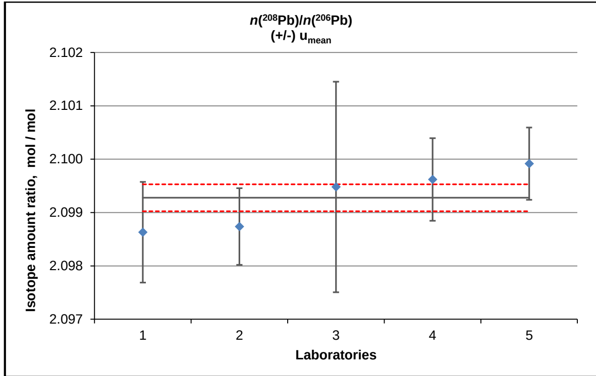
Figure A4.7. Interlaboratory study results for characterization of n(^{208}\text{Pb})/n(^{206}\text{Pb})
