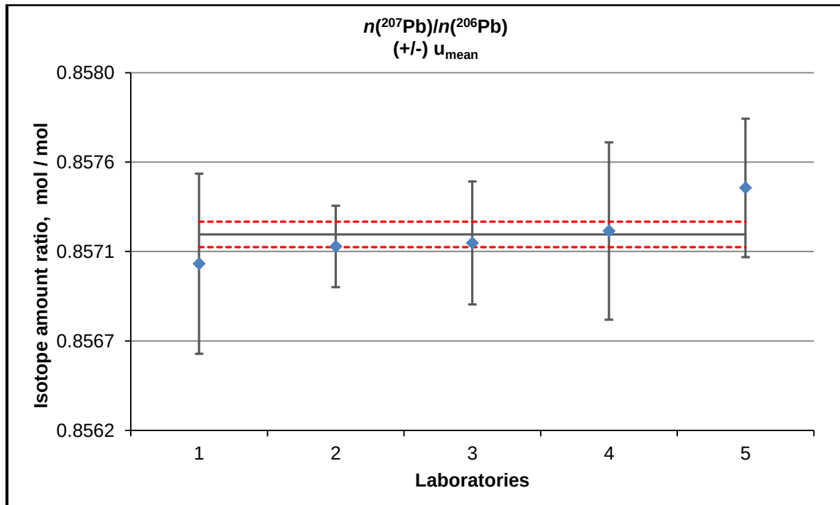
Figure A4.6. Interlaboratory study results for characterization of n(^{207}\text{Pb})/n(^{206}\text{Pb})
