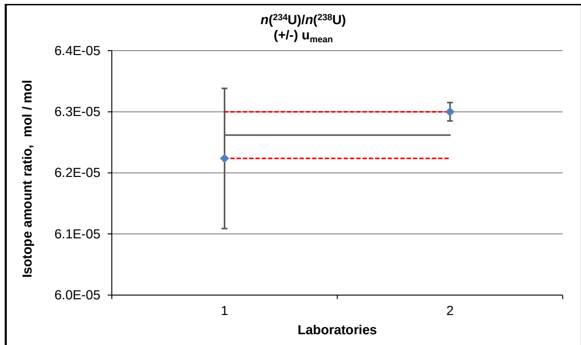
Figure A4.8. Interlaboratory study results for characterization of n(^{234}\text{U})/n(^{238}\text{U})
