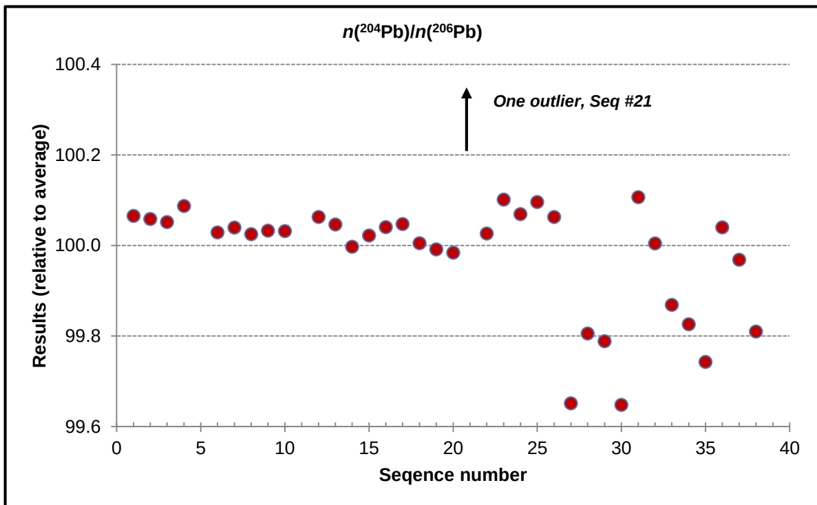
Figure A1.5. Homogeneity graphs for n(^{204}\text{Pb})/n(^{206}\text{Pb})
