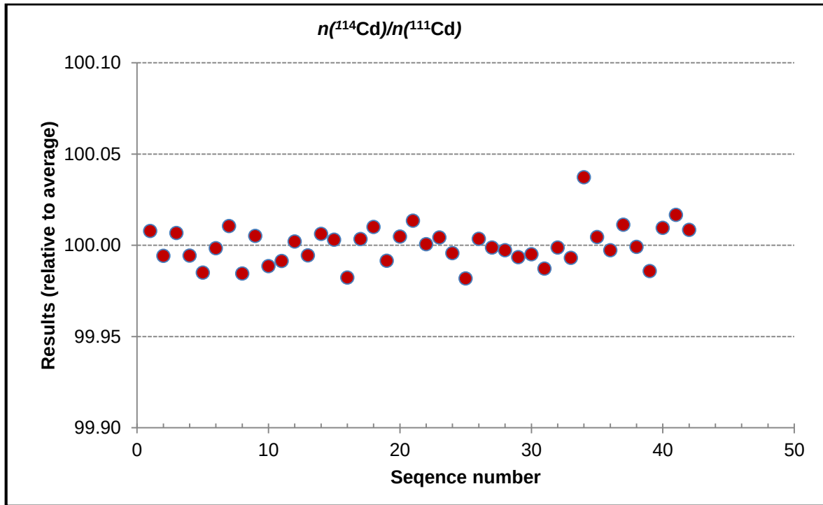
Figure A1.3. Homogeneity graphs for n(^{114}\text{Cd})/n(^{111}\text{Cd})
