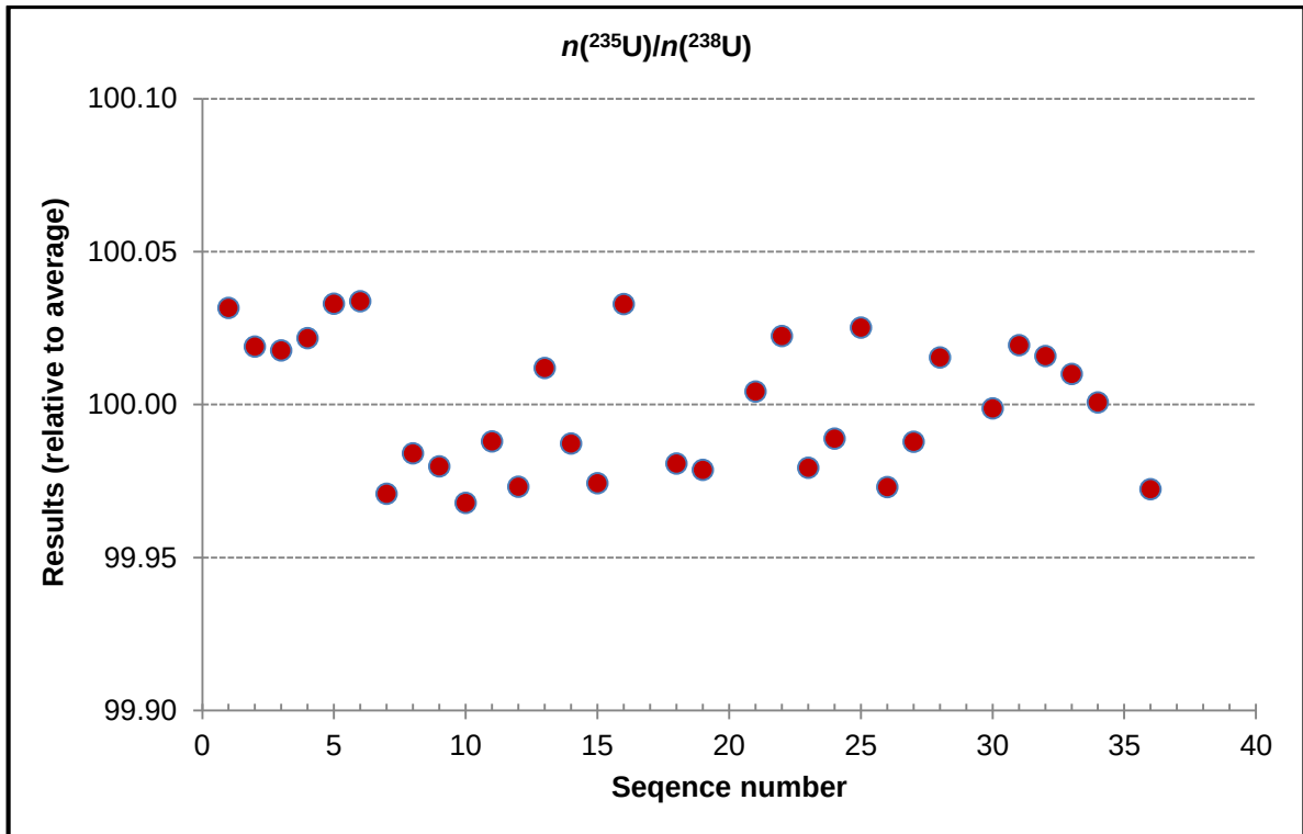
Figure A1.9. Homogeneity graphs for n(^{235}\text{U})/n(^{238}\text{U})
