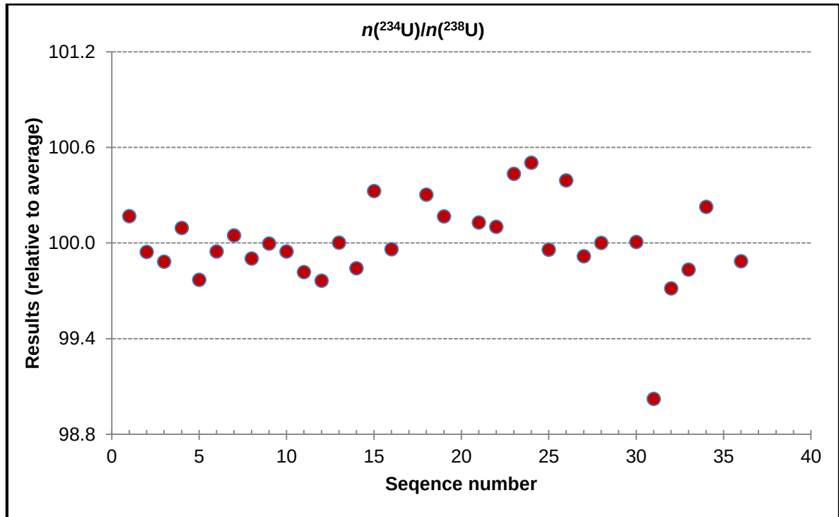
Figure A1.8. Homogeneity graphs for n(^{234}\text{U})/n(^{238}\text{U})
