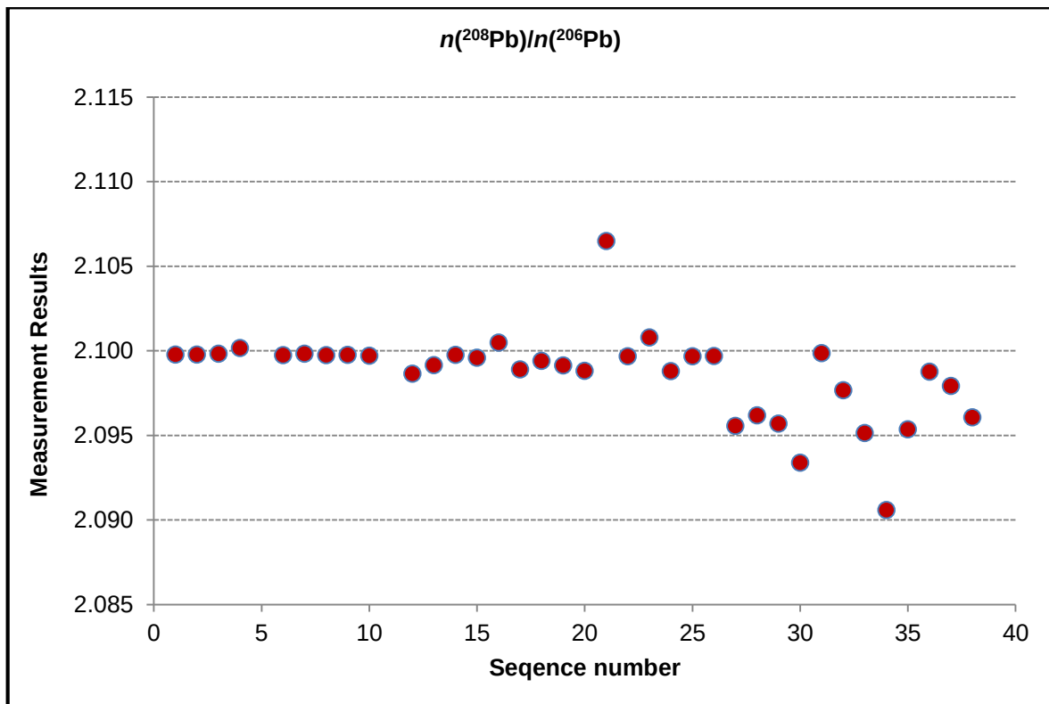
Figure A3.7. Long-term stability at +21 °C for n(^{208}\text{Pb})/n(^{206}\text{Pb})
