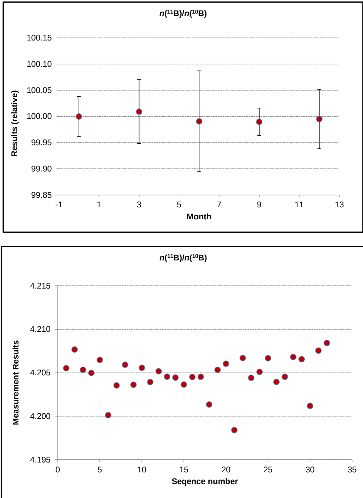
Figure A3.1. Long-term stability at +21 °C for n(^{11}\text{B})/n(^{10}\text{B})
