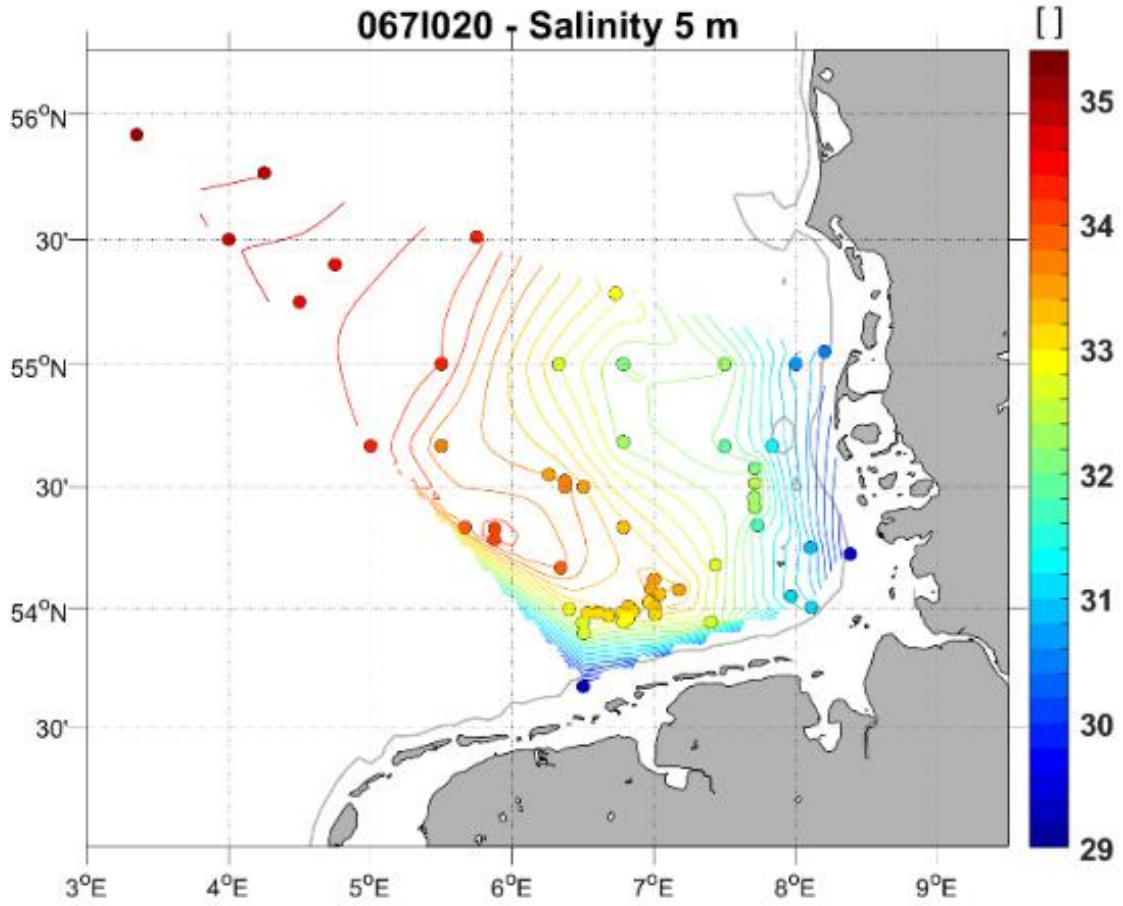
Figure 4. Salinity ( g \cdot kg^{-1} ) measured at a depth of 5 m at different sampling locations
