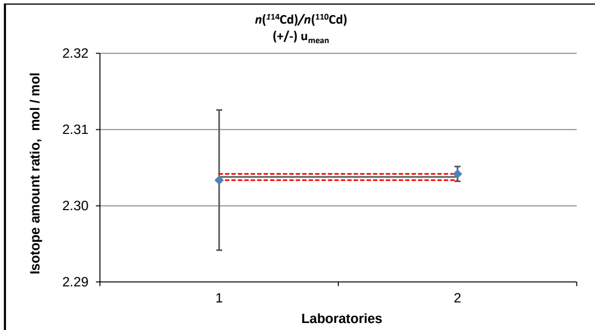
Figure A4.2. Interlaboratory study results for characterization of n(^{114}\text{Cd})/n(^{110}\text{Cd})
