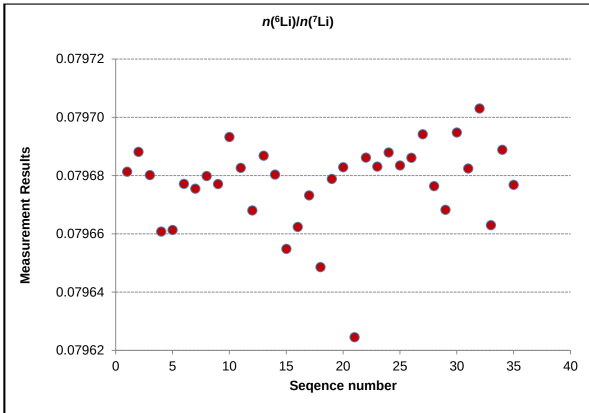
Figure A3.4. Long-term stability at +21 °C for n(^6\text{Li})/n(^7\text{Li})
