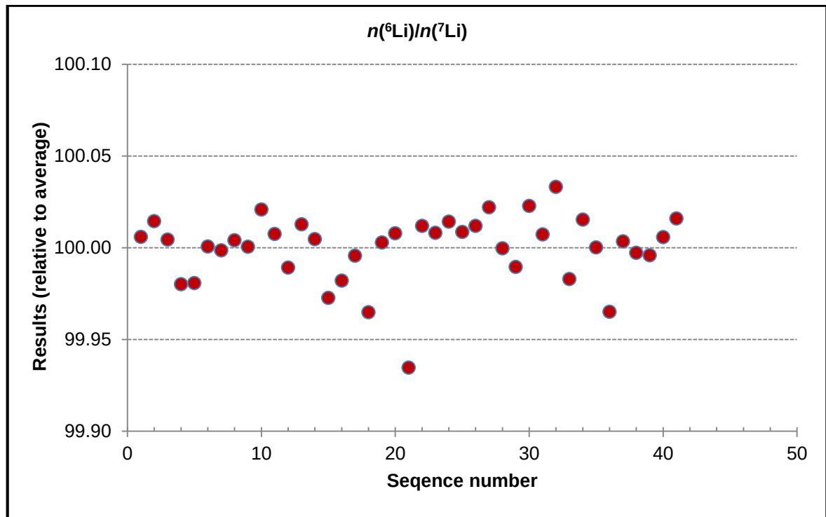
Figure A1.4. Homogeneity graphs for n(^7\text{Li})/n(^6\text{Li}) .
