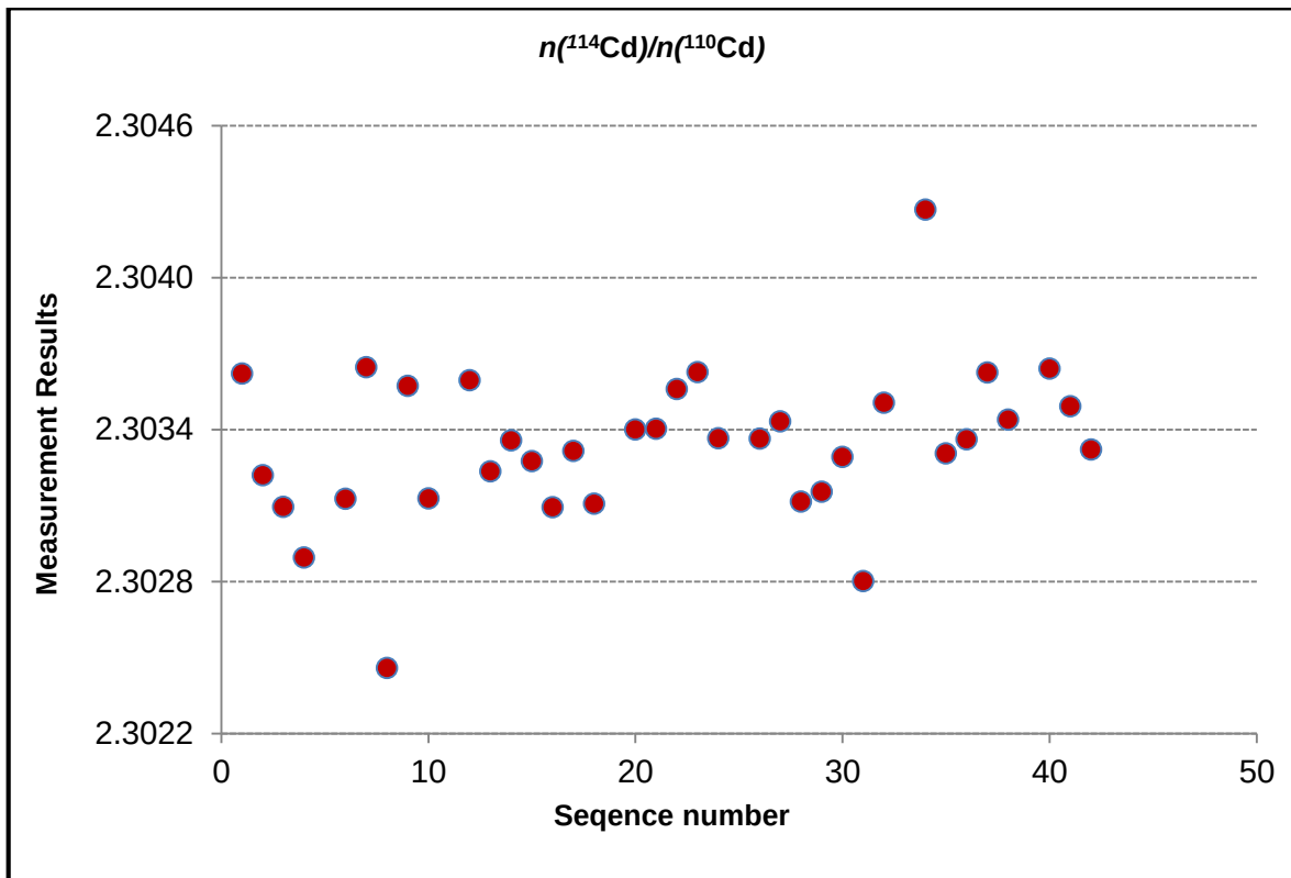
Figure A3.2. Long-term stability at +21 °C for n(^{114}\text{Cd})/n(^{110}\text{Cd})
