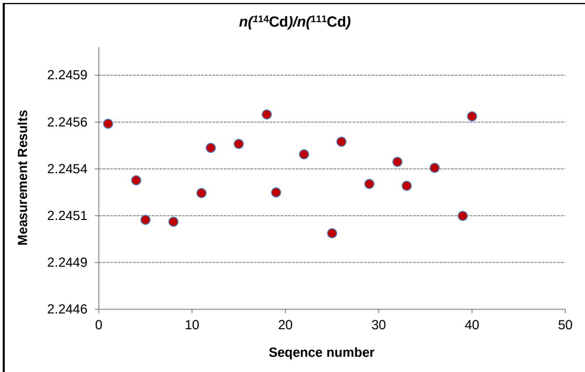
Figure A2.3. Short-term stability at +45 °C for n(^{114}\text{Cd})/n(^{111}\text{Cd})
