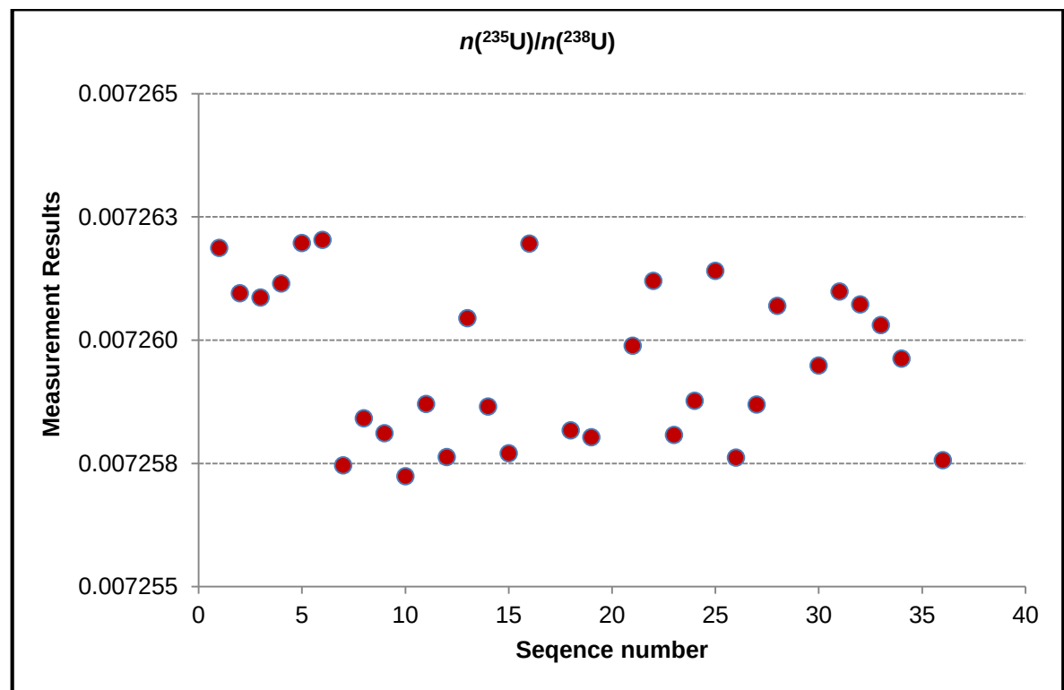
Figure A3.9. Long-term stability at +21 °C for °C for n(^{235}\text{U})/n(^{238}\text{U})
