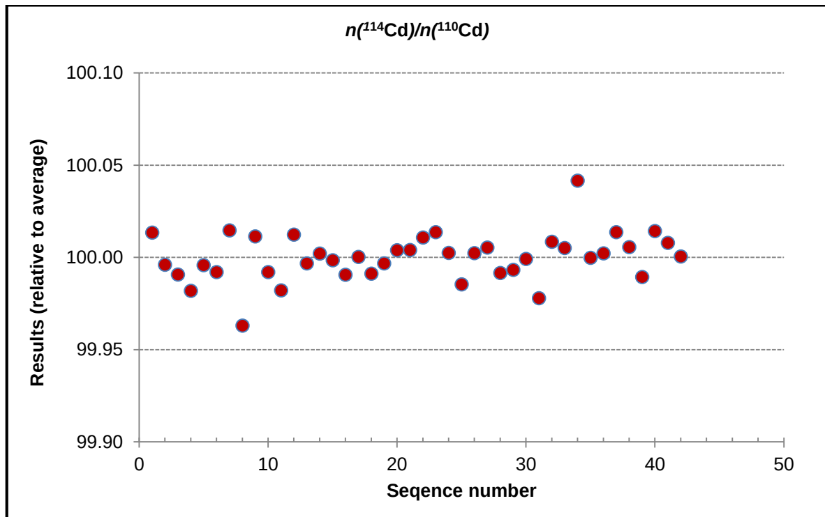
Figure A1.2. Homogeneity graphs for n(^{114}\text{Cd})/n(^{110}\text{Cd})
