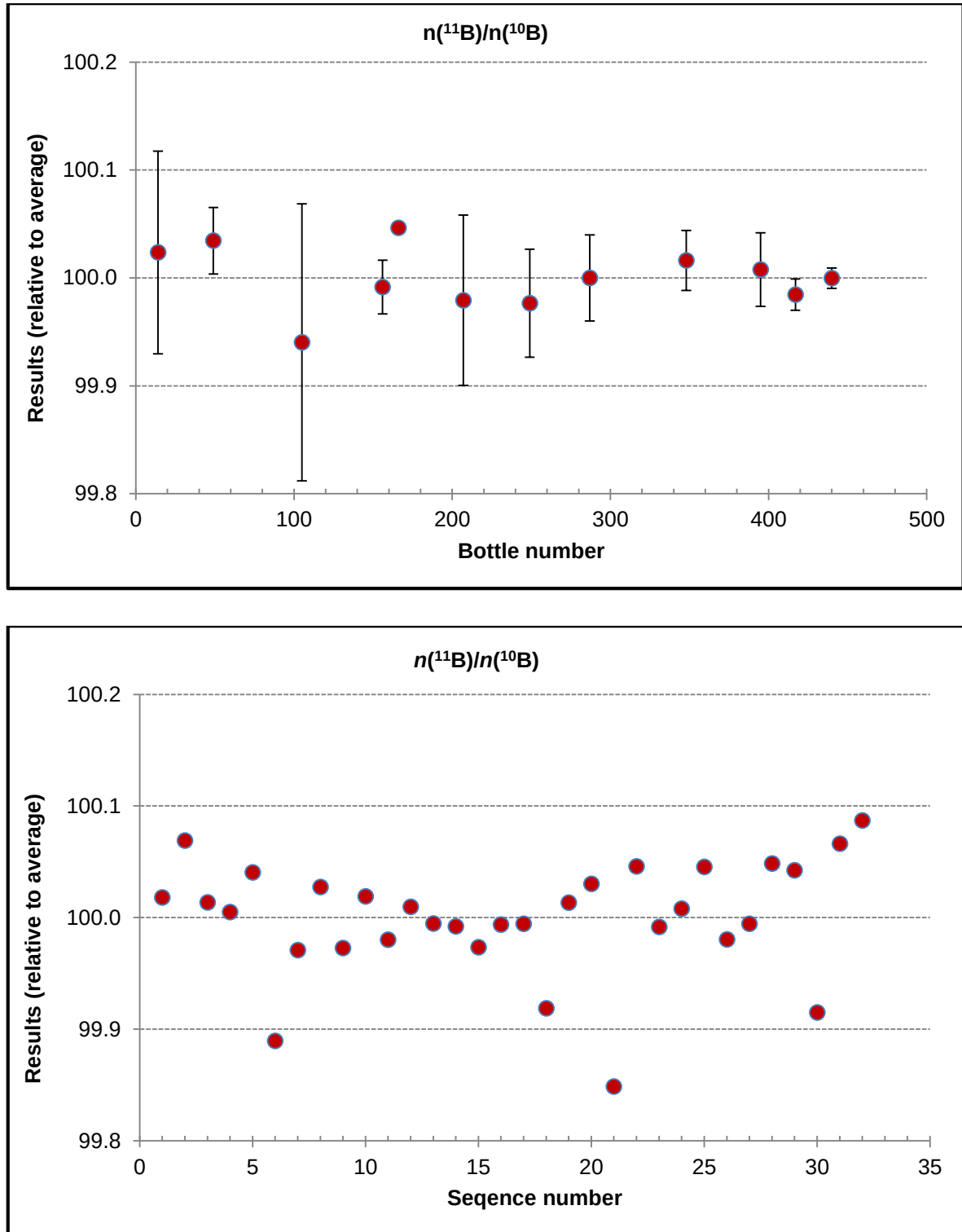
Figure A1.1. Homogeneity graphs for n(^{11}\text{B})/n(^{10}\text{B})
